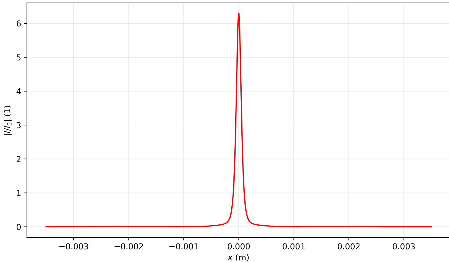
Intensity profile I(x, y = 0, z = 1.274)/I_0 , P_{in}=5.0P_{cr} , artificial time
